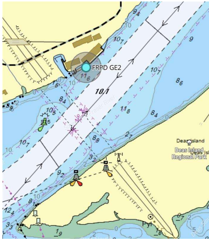
Figure 2: Marine Equipment Staging (Nautical Chart)
