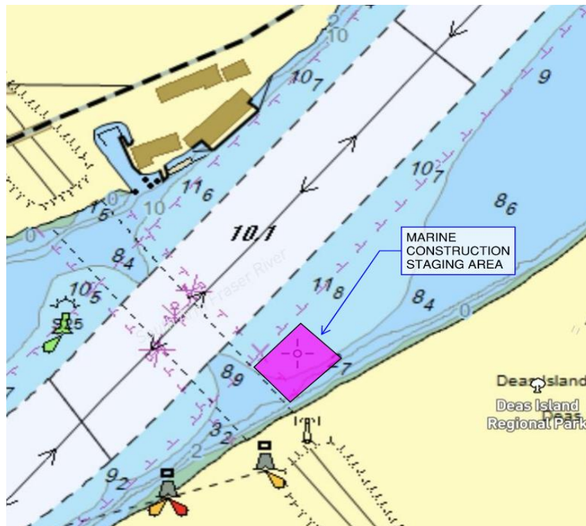
Figure 1: Marine Staging Equipment
