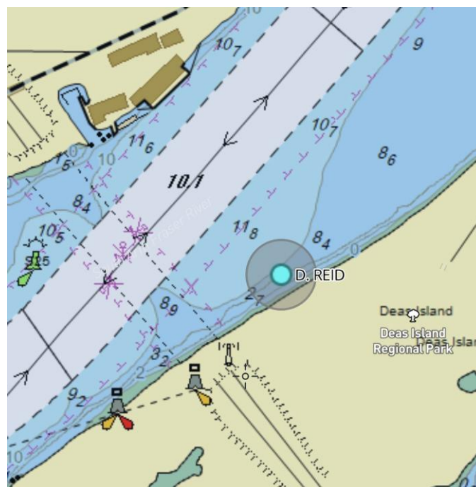
Figure 4: Marine Construction Equipment - D. Reid Marine Derrick - Location
