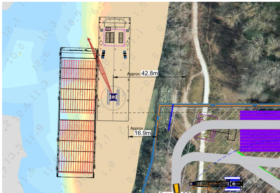
Figure 1: Marine Staging Equipment
