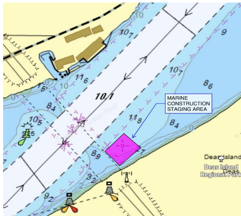
Figure 2: Marine Construction Staging Area
