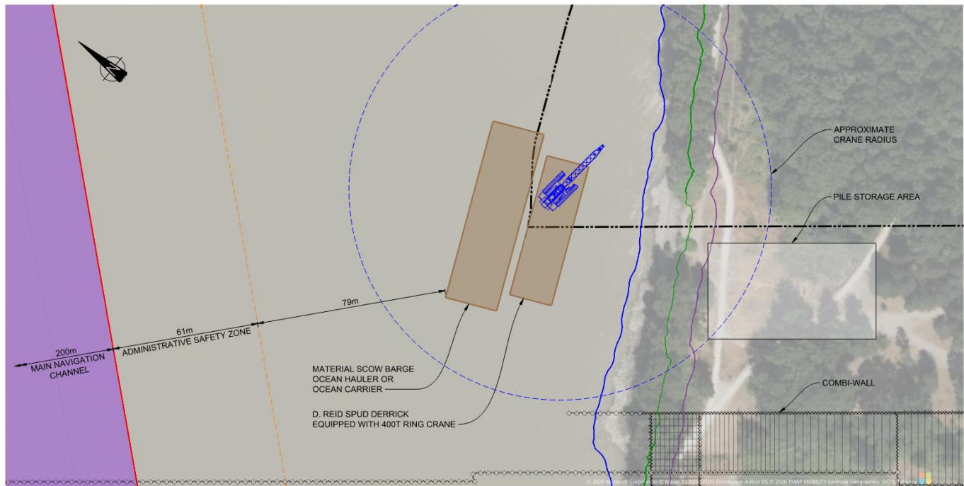
Figure 3: Marine Construction Staging Area
