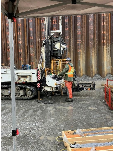
Figure 2: Ground-densification testing on Deas Island (Dec. 8, 2025).
