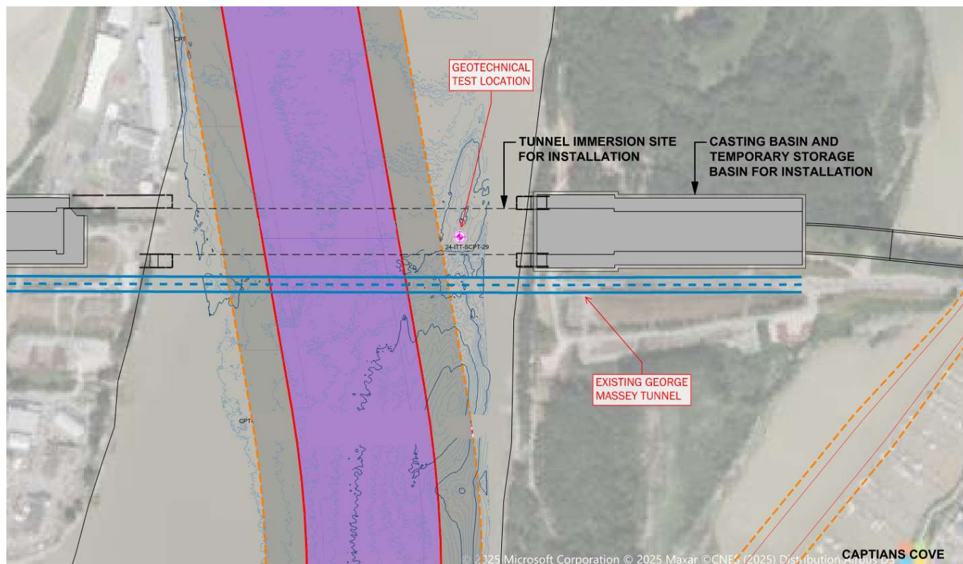
Figure 3: Geotechnical Drilling Location
