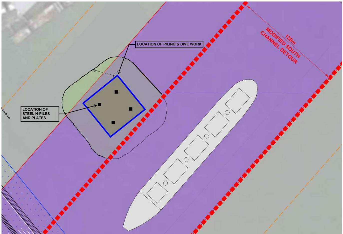
Figure 3: Test Area (Supplemental Test Dredge Area)
