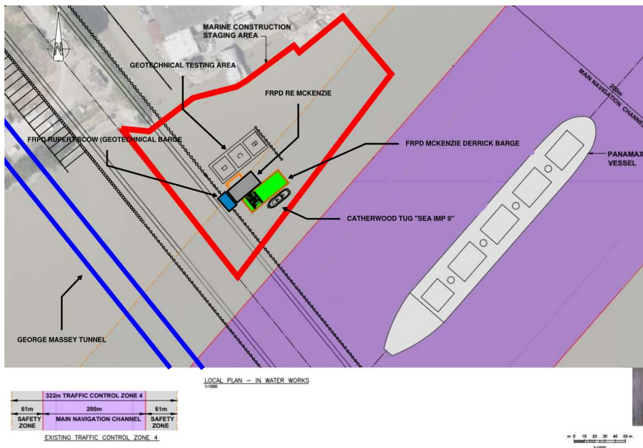
Figure 1: Geotechnical Testing
