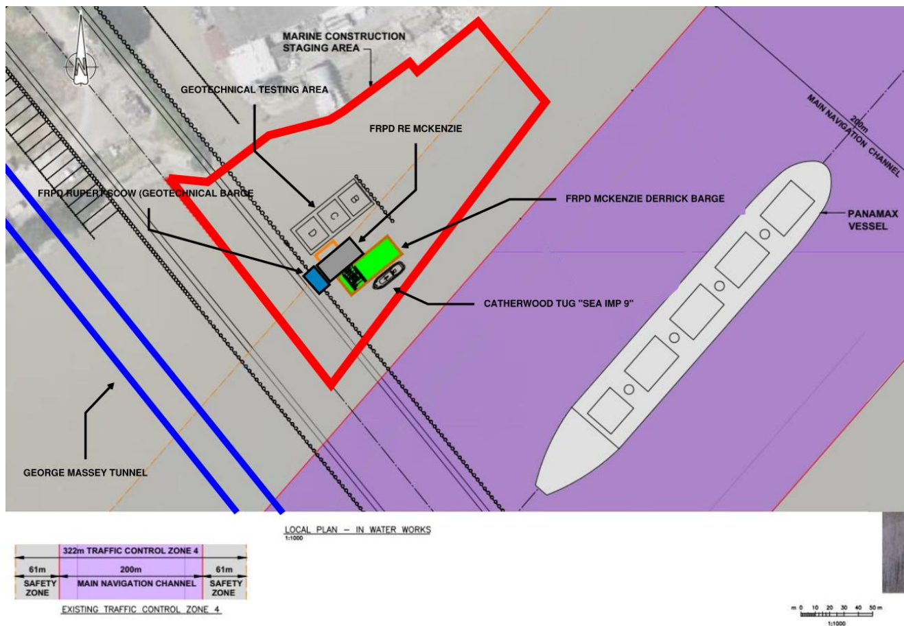
Figure 1: Geotechnical Testing
