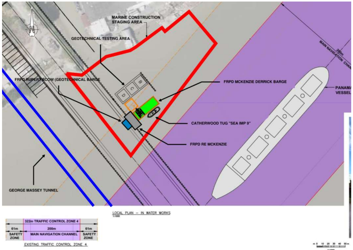
Figure 1: Geotechnical Testing
