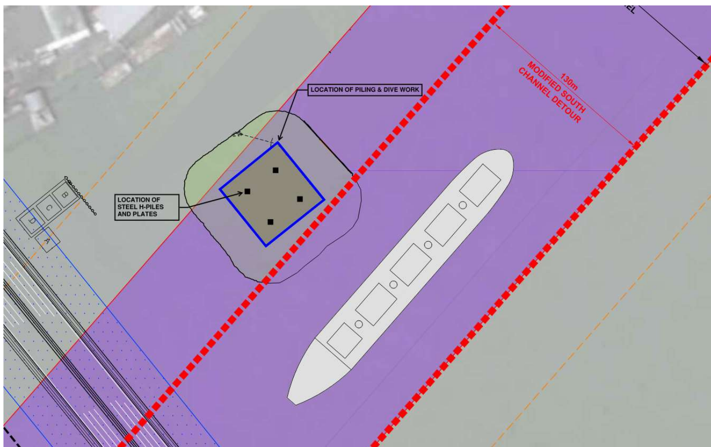
Figure 1: Equipment Positioning & Modified South Channel Detour
