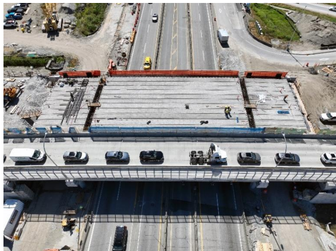
Phase 2 girders in place next to traffic flowing on the completed Phase 1 structure (August 11, 2025).
