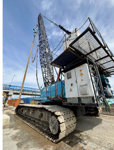
Figure 2: Heavy lift crane used for Phase 2 stone column work in the southwest quadrant.
