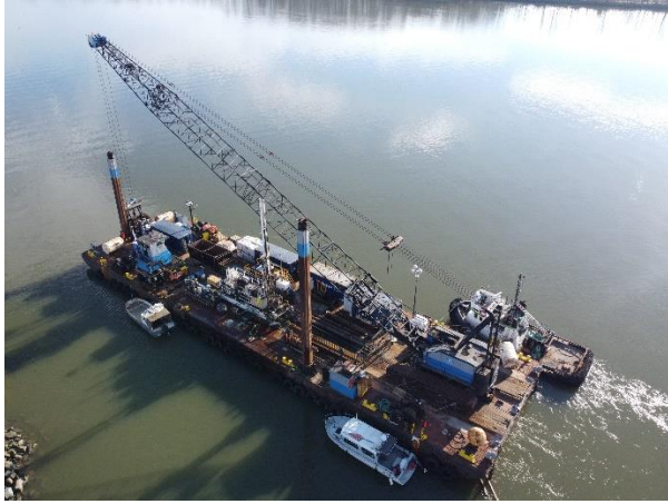
Figure 1: A close-up picture of the barge from which the marine geotechnical investigations were carried out.
