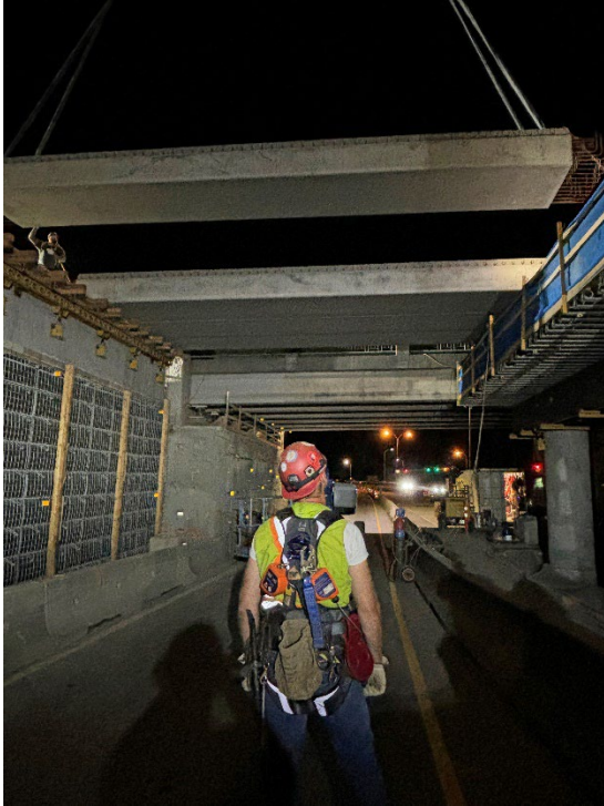
Image 1: Workers manoeuvre east side end-span girders into position on the Phase 1 overpass.
