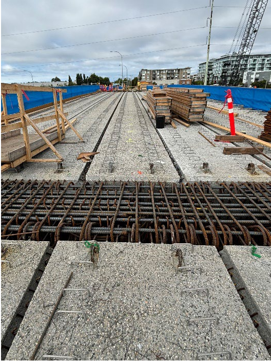
Image 3: Phase 1 deck construction underway facing west
