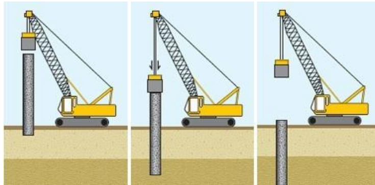
A visual of pile driving being completed with machinery.
